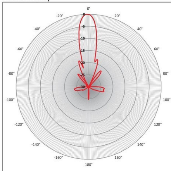
Directionality
