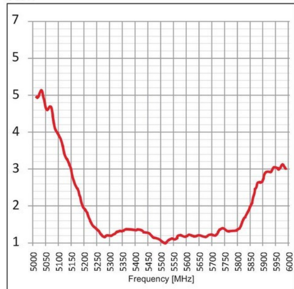
SWR
