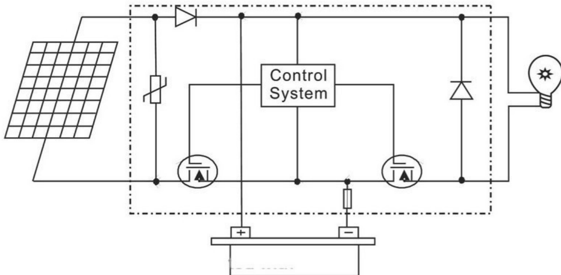
Principle Diagram of the Controller
